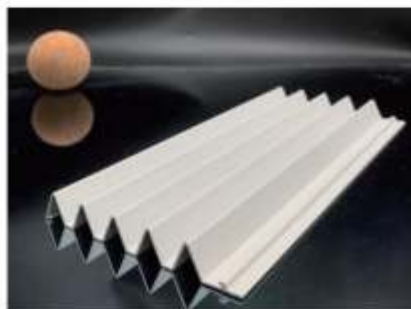
B37 Great Wall plate series -B37 size6000*100*27.1mm
