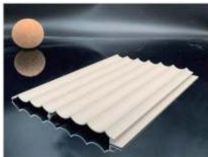
B53 Arc Series -B53 size6000*140*10.9mm
