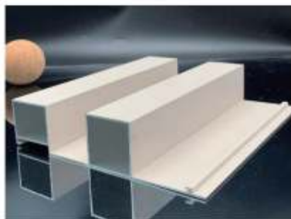
B18 Great Wall plate series -B18 size6000*161.4*40mm
